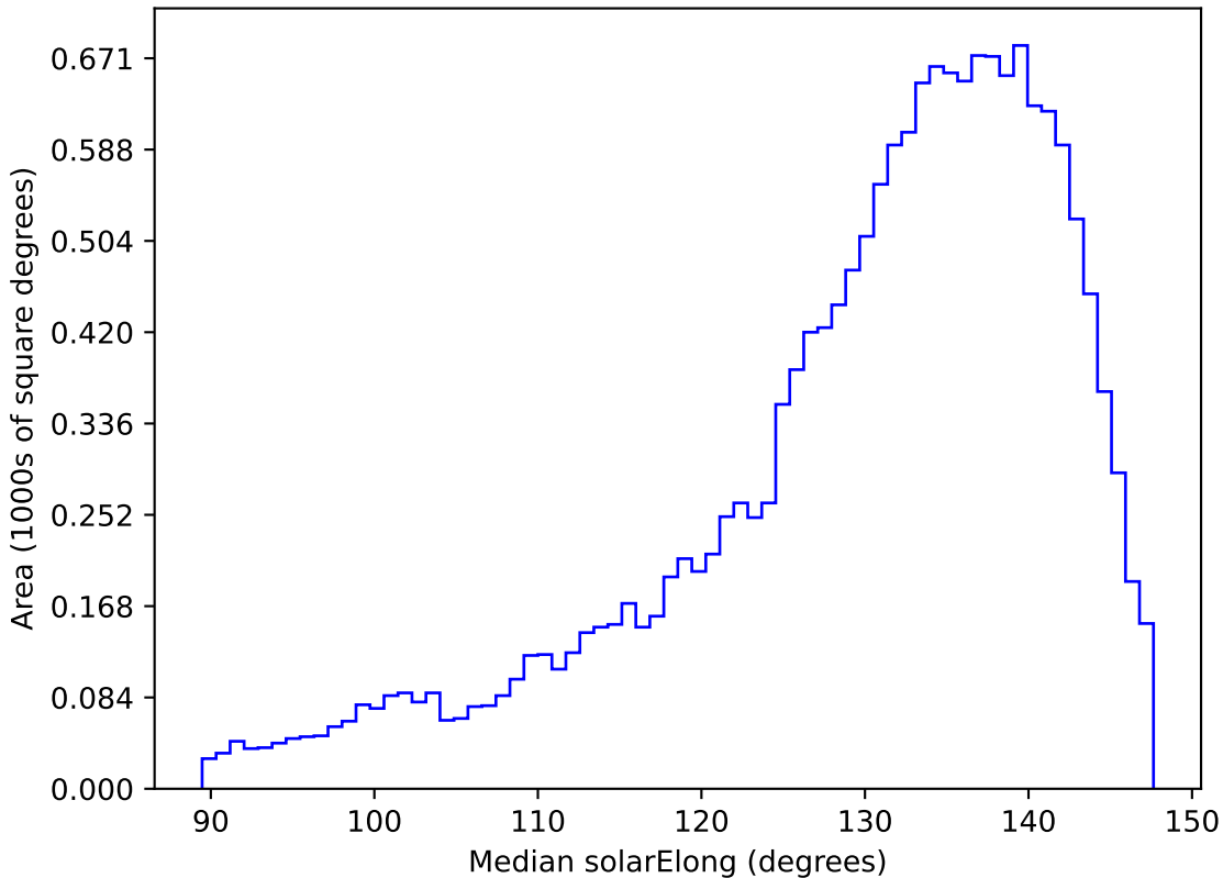
ddf_loaded_half_fl4_v3.4_10yrs WFD y band: Median solarElong
