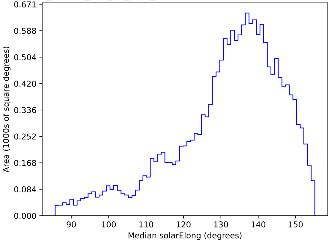
ddf_loaded_half_fl4_v3.4_10yrs WFD u band: Median solarElong
