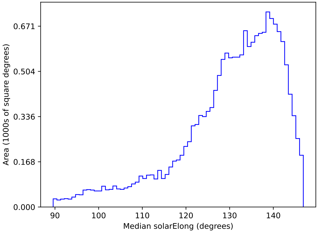
ddf_loaded_half_fl4_v3.4_10yrs WFD r band: Median solarElong
