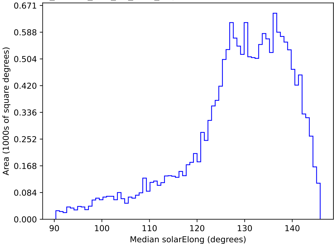
ddf_loaded_half_fl4_v3.4_10yrs WFD i band: Median solarElong
