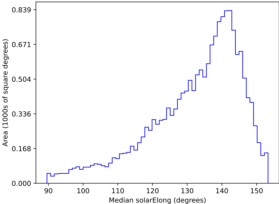
ddf_loaded_half_fl4_v3.4_10yrs WFD g band: Median solarElong
