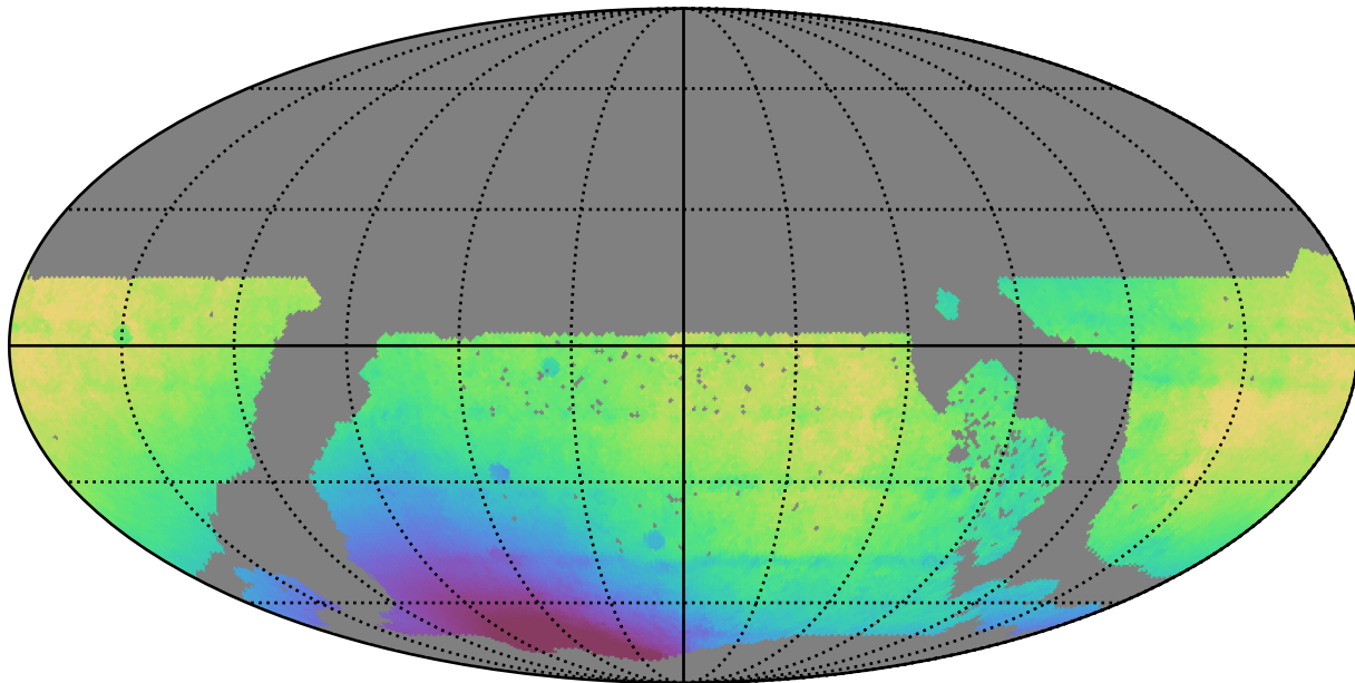
ddf_loaded_half_fl4_v3.4_10yrs WFD all bands: Median solarElong
