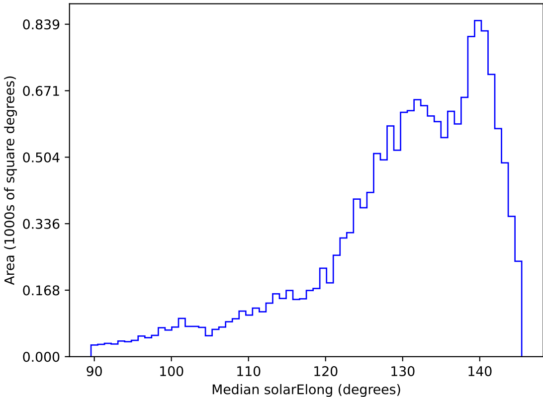
ddf_loaded_half_fl4_v3.4_10yrs WFD all bands: Median solarElong
