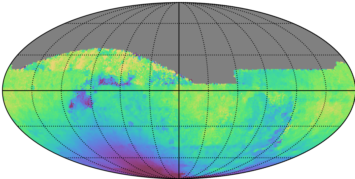
ddf_loaded_half_fl4_v3.4_10yrs All sky z band: Median solarElong
