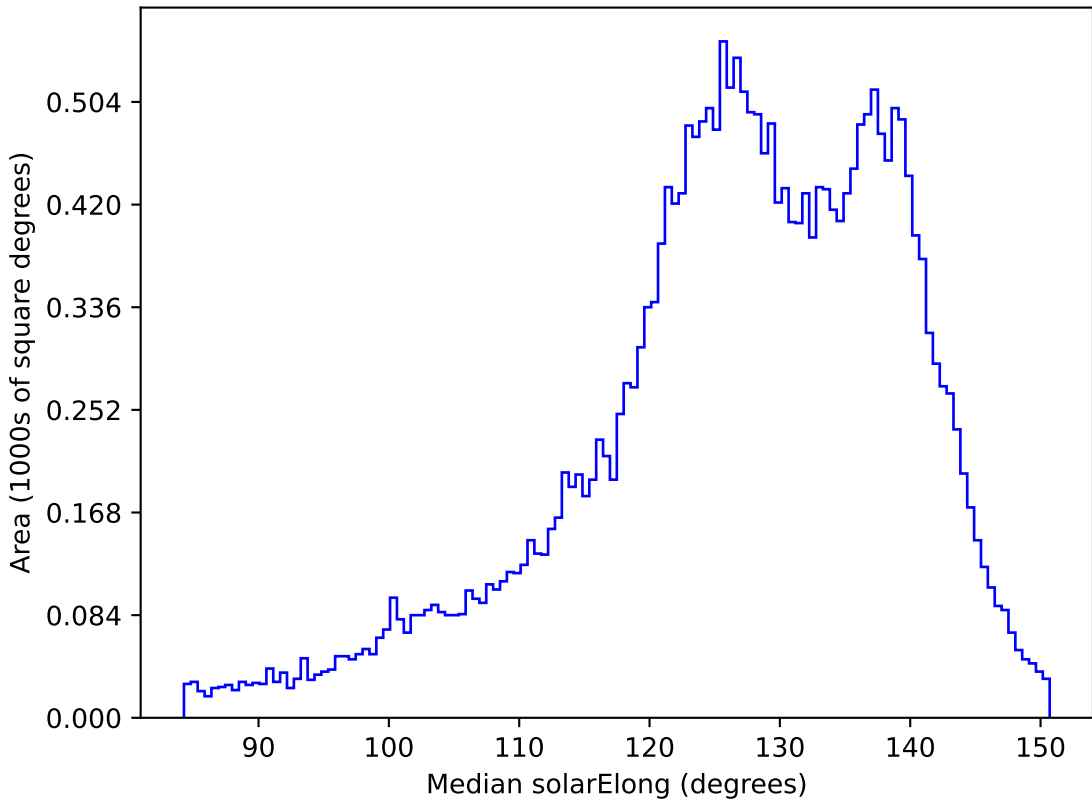
ddf_loaded_half_fl4_v3.4_10yrs All sky z band: Median solarElong
