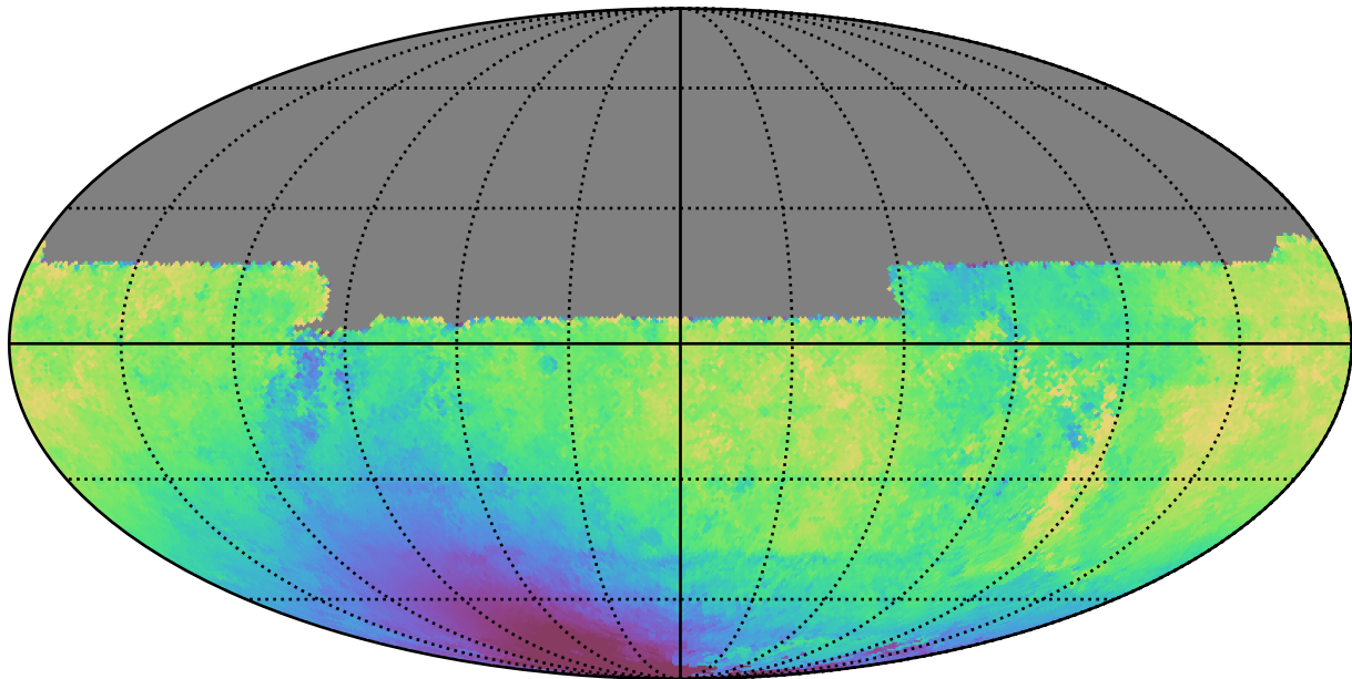
ddf_loaded_half_fl4_v3.4_10yrs All sky y band: Median solarElong
