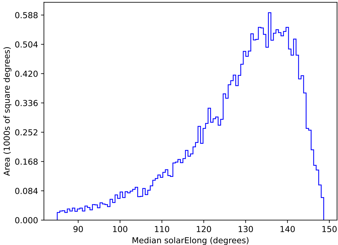
ddf_loaded_half_fl4_v3.4_10yrs All sky y band: Median solarElong
