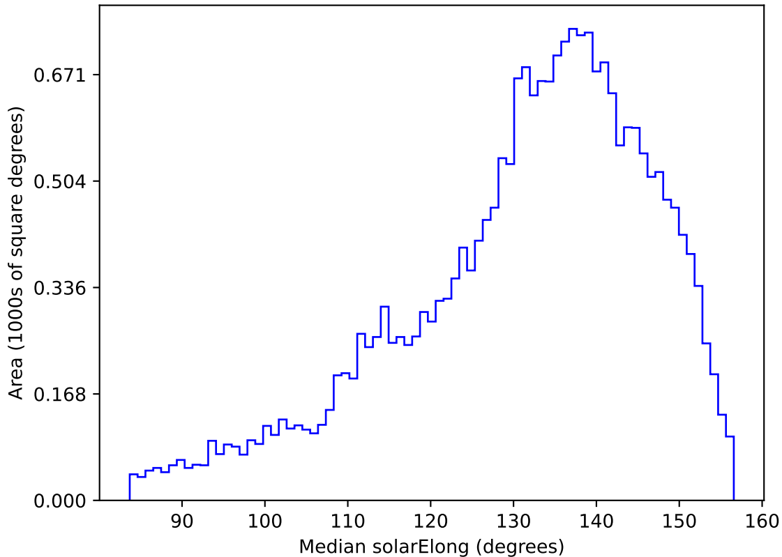
ddf_loaded_half_fl4_v3.4_10yrs All sky u band: Median solarElong
