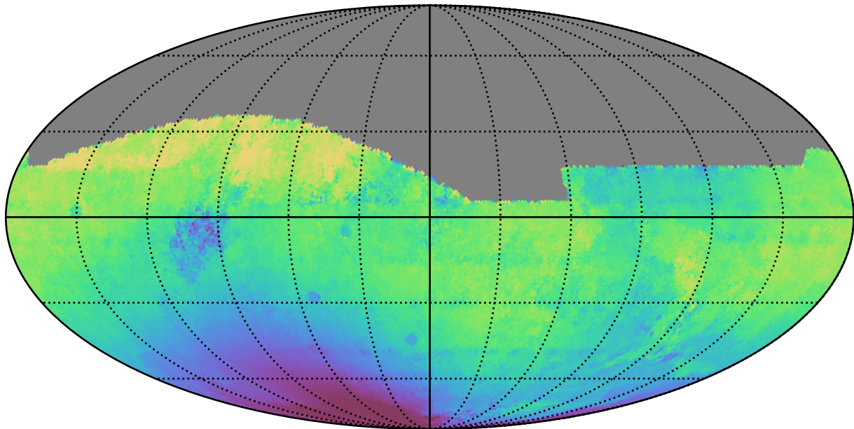
ddf_loaded_half_fl4_v3.4_10yrs All sky r band: Median solarElong
