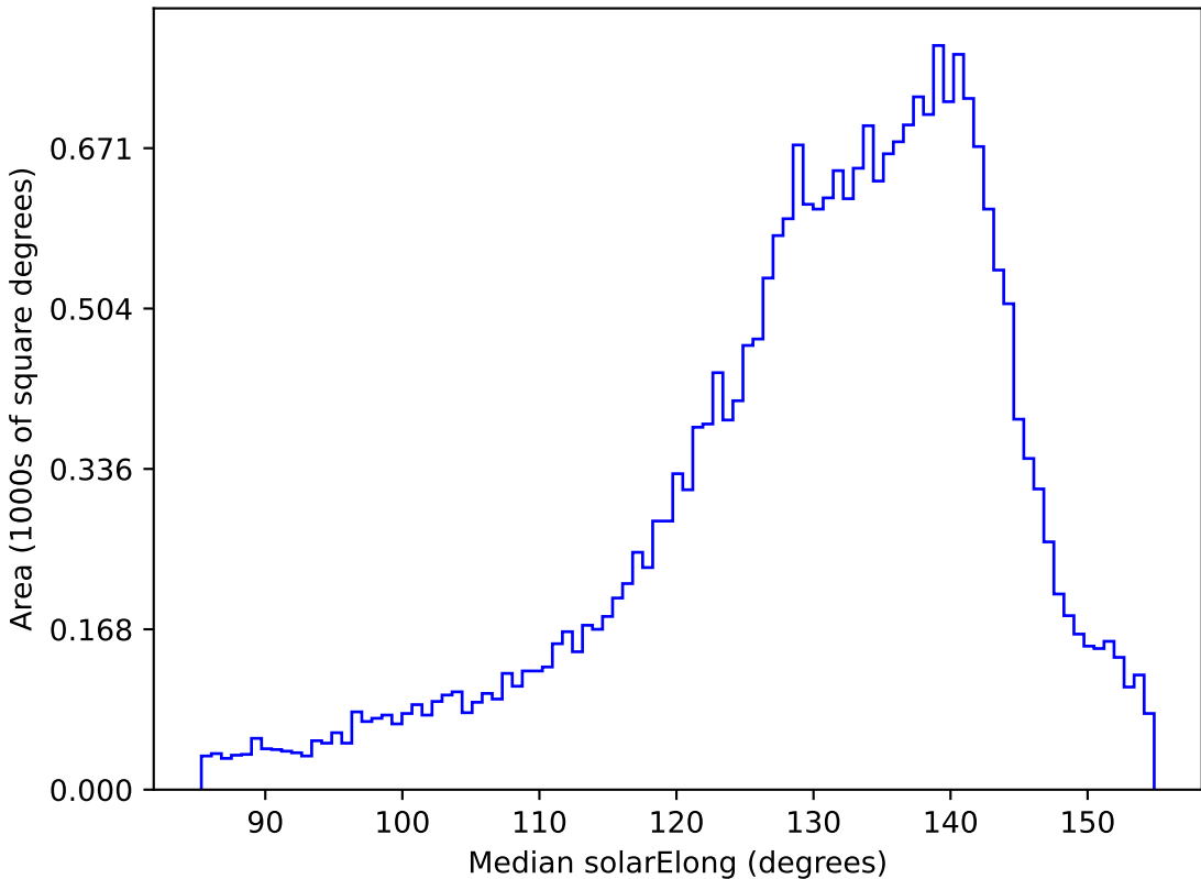
ddf_loaded_half_fl4_v3.4_10yrs All sky r band: Median solarElong
