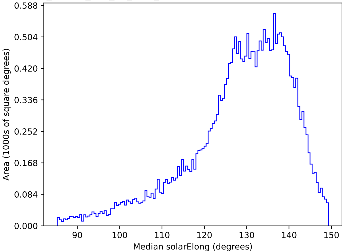
ddf_loaded_half_fl4_v3.4_10yrs All sky i band: Median solarElong
