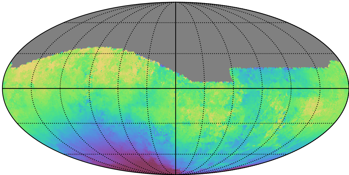
ddf_loaded_half_fl4_v3.4_10yrs All sky g band: Median solarElong
