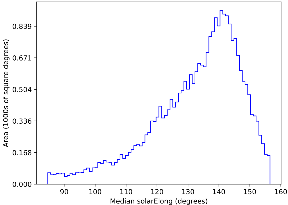
ddf_loaded_half_fl4_v3.4_10yrs All sky g band: Median solarElong
