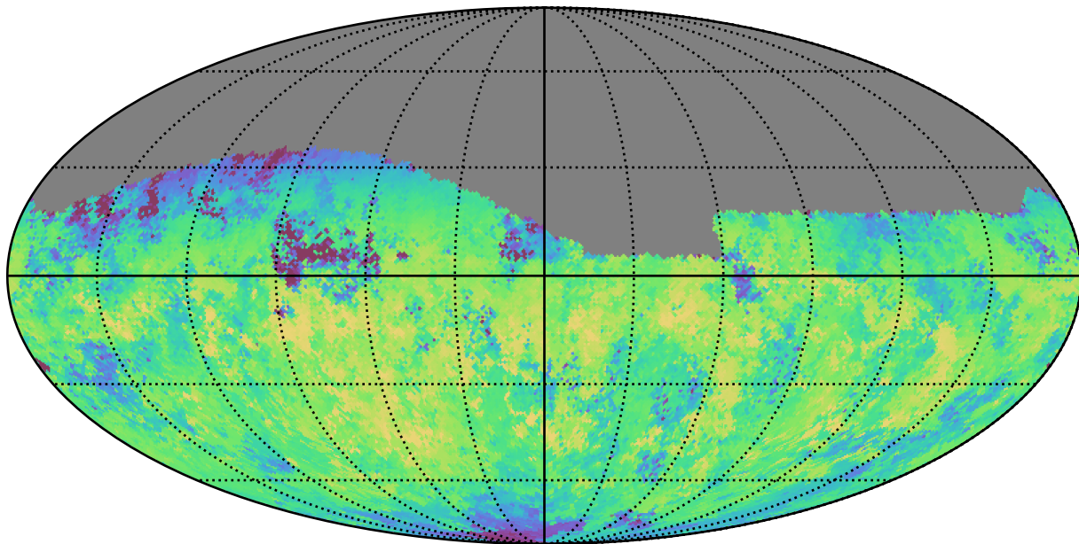
ddf_loaded_half_fl4_v3.4_10yrs Yr 1 z band: Median skyBrightness
