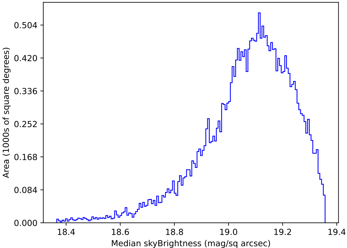
ddf_loaded_half_fl4_v3.4_10yrs Yr 1 z band: Median skyBrightness
