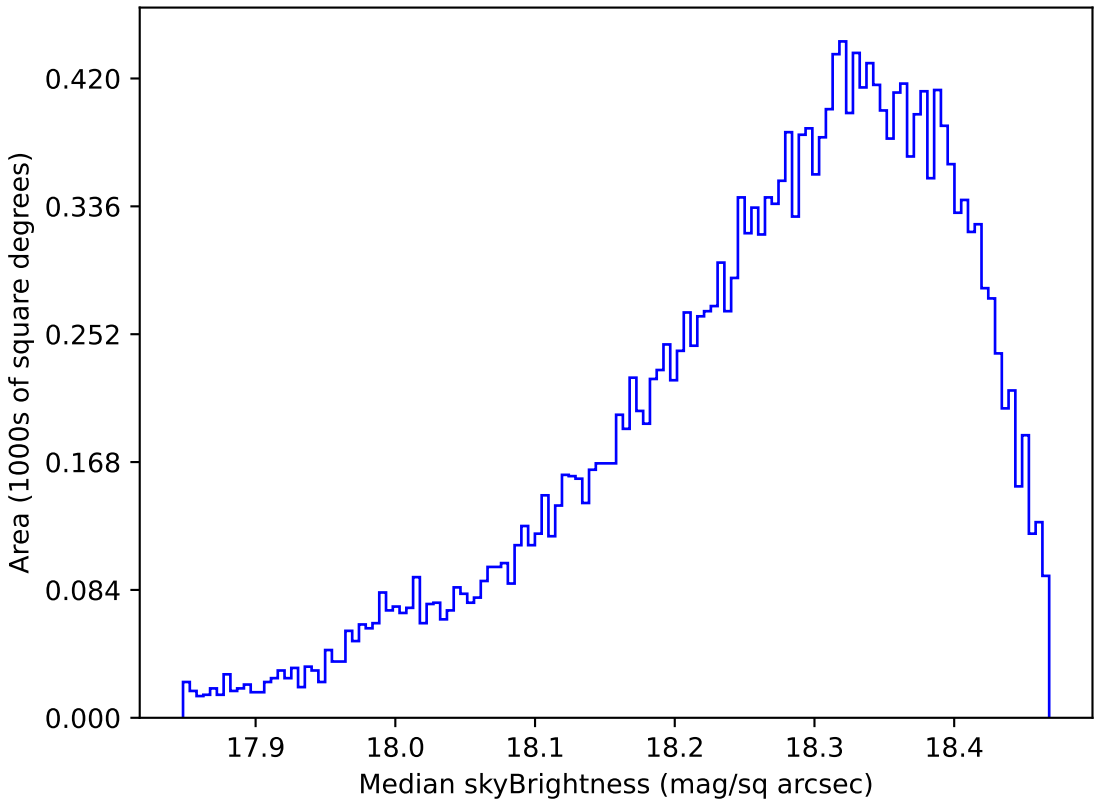
ddf_loaded_half_fl4_v3.4_10yrs Yr 1 y band: Median skyBrightness
