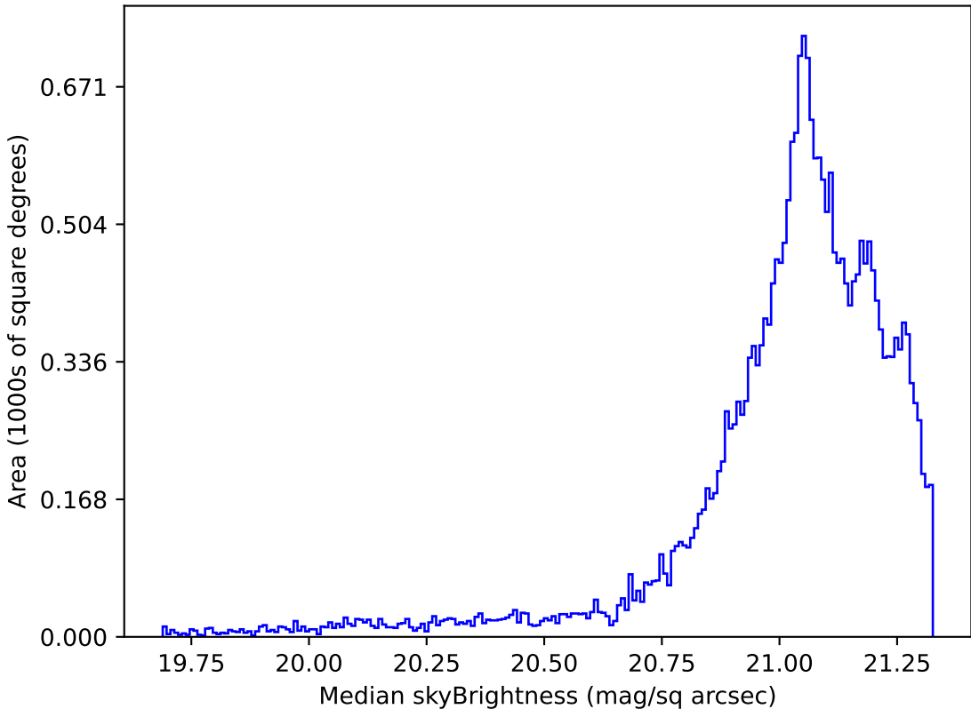
ddf_loaded_half_fl4_v3.4_10yrs Yr 1 r band: Median skyBrightness
