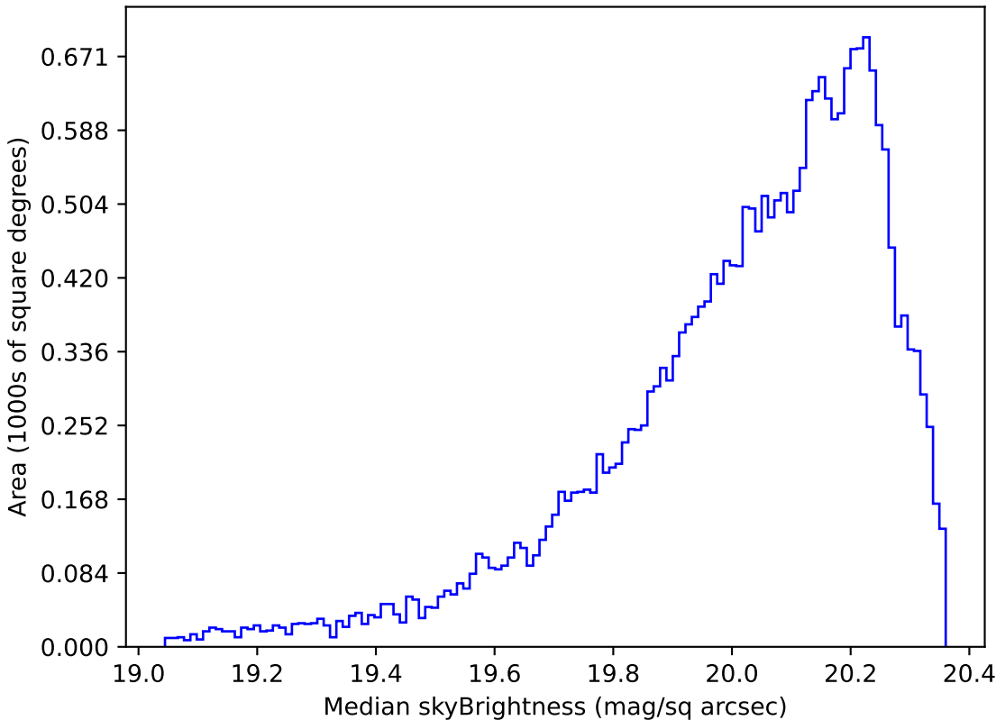
ddf_loaded_half_fl4_v3.4_10yrs Yr 1 i band: Median skyBrightness
