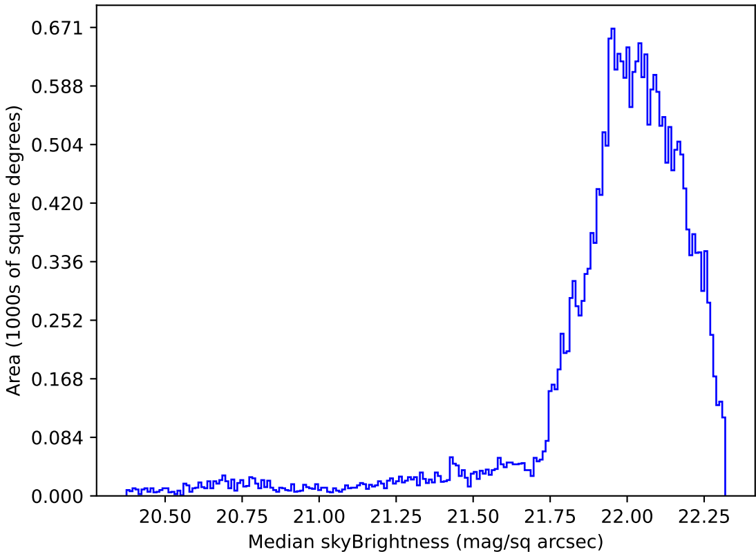
ddf_loaded_half_fl4_v3.4_10yrs Yr 1 g band: Median skyBrightness
