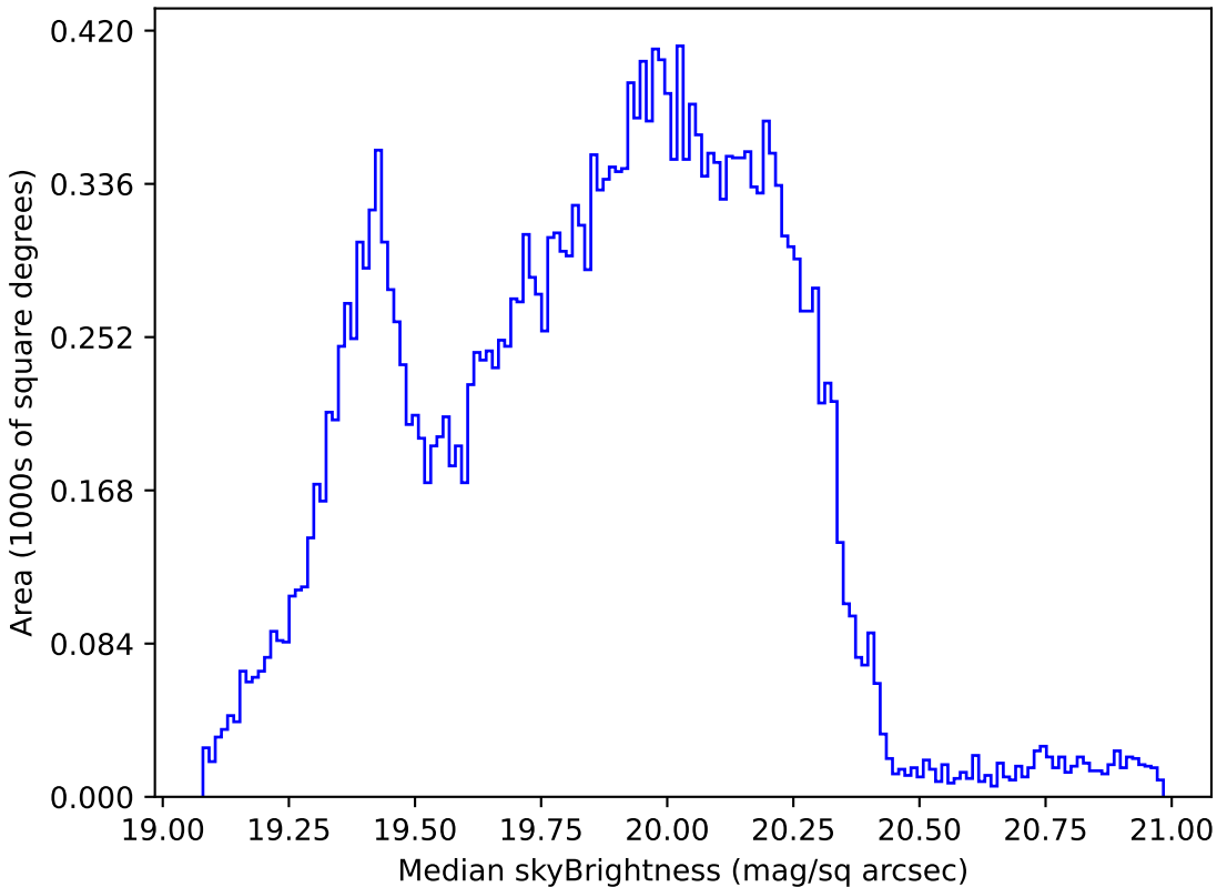
ddf_loaded_half_fl4_v3.4_10yrs Yr 1 all bands: Median skyBrightness
