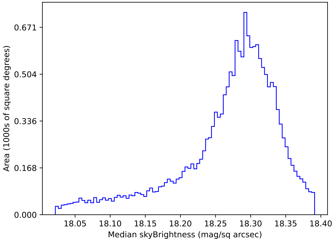
ddf_loaded_half_fl4_v3.4_10yrs WFD y band: Median skyBrightness
