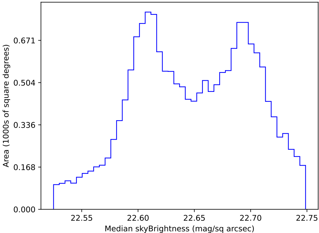
ddf_loaded_half_fl4_v3.4_10yrs WFD u band: Median skyBrightness
