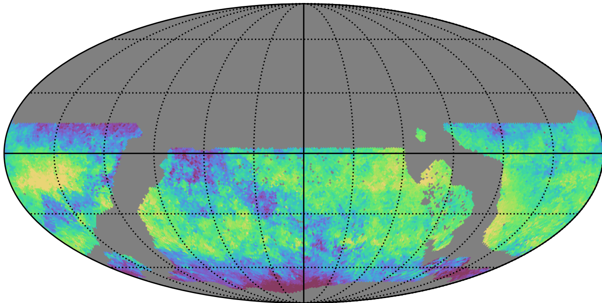
ddf_loaded_half_fl4_v3.4_10yrs WFD i band: Median skyBrightness
