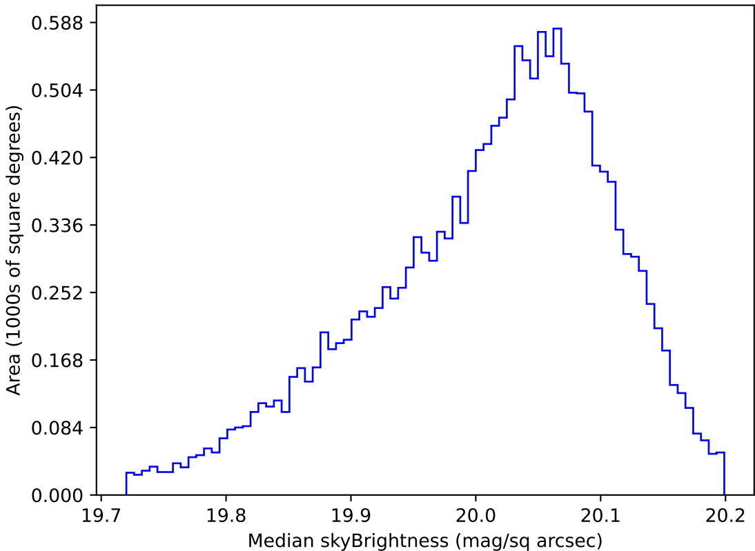
ddf_loaded_half_fl4_v3.4_10yrs WFD i band: Median skyBrightness
