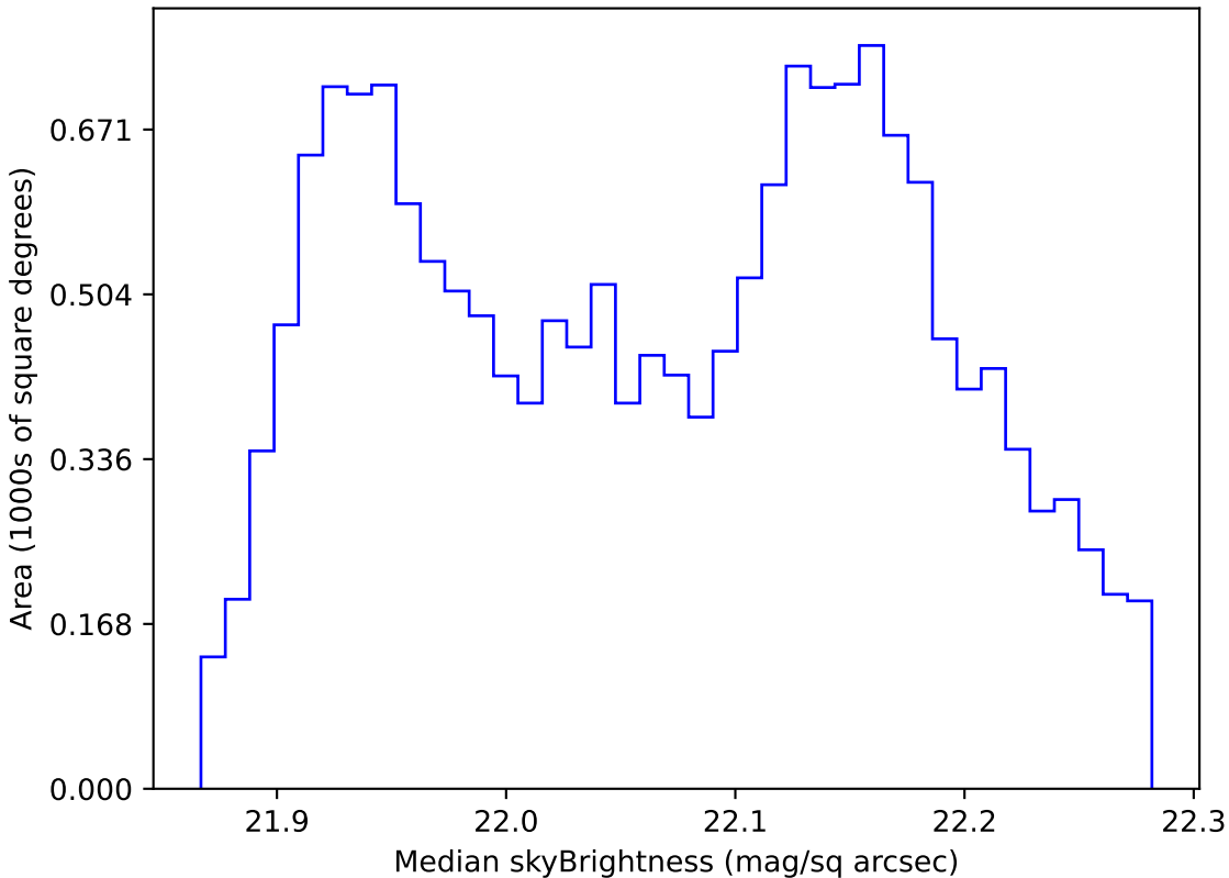
ddf_loaded_half_fl4_v3.4_10yrs WFD g band: Median skyBrightness
