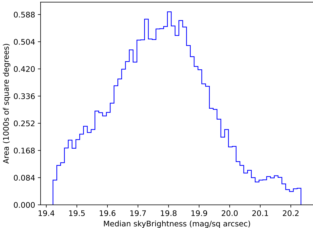
ddf_loaded_half_fl4_v3.4_10yrs WFD all bands: Median skyBrightness
