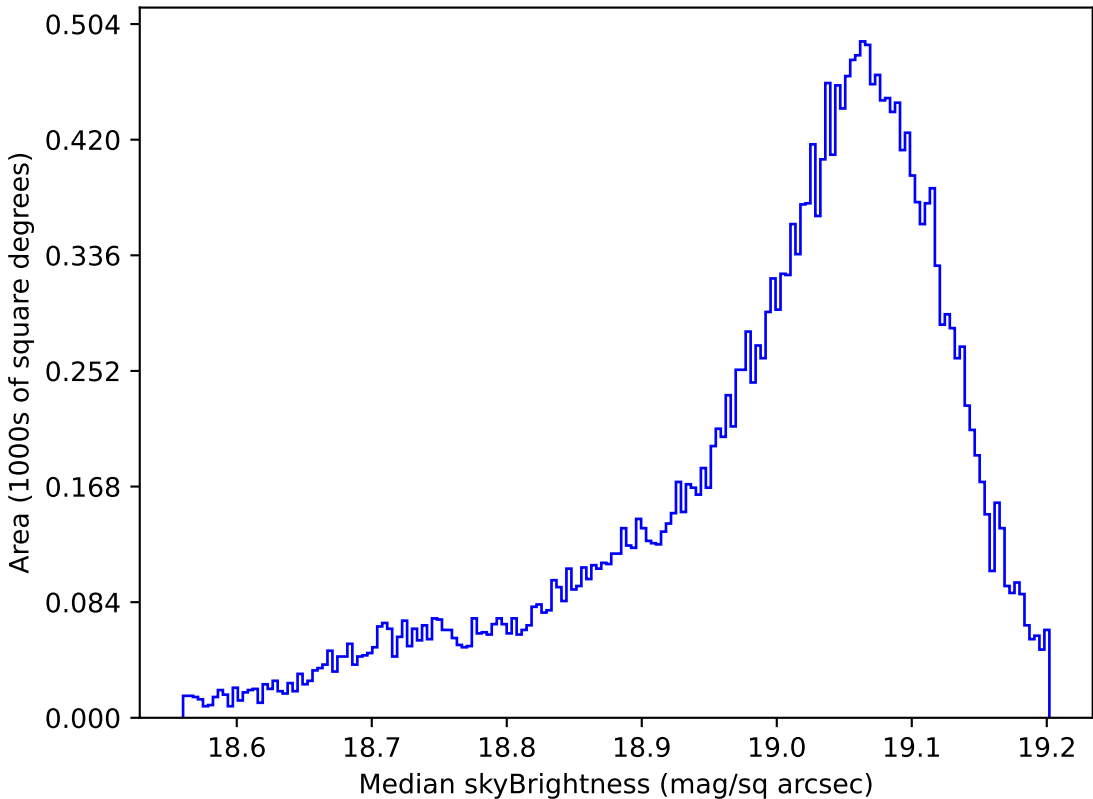
ddf_loaded_half_fl4_v3.4_10yrs All sky z band: Median skyBrightness
