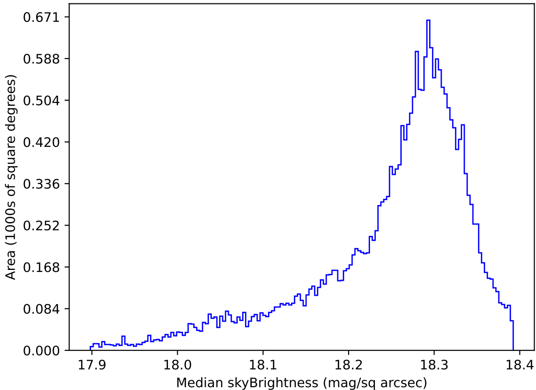
ddf_loaded_half_fl4_v3.4_10yrs All sky y band: Median skyBrightness
