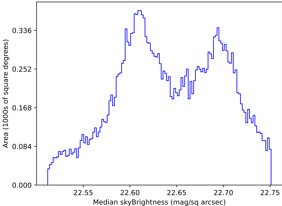
ddf_loaded_half_fl4_v3.4_10yrs All sky u band: Median skyBrightness
