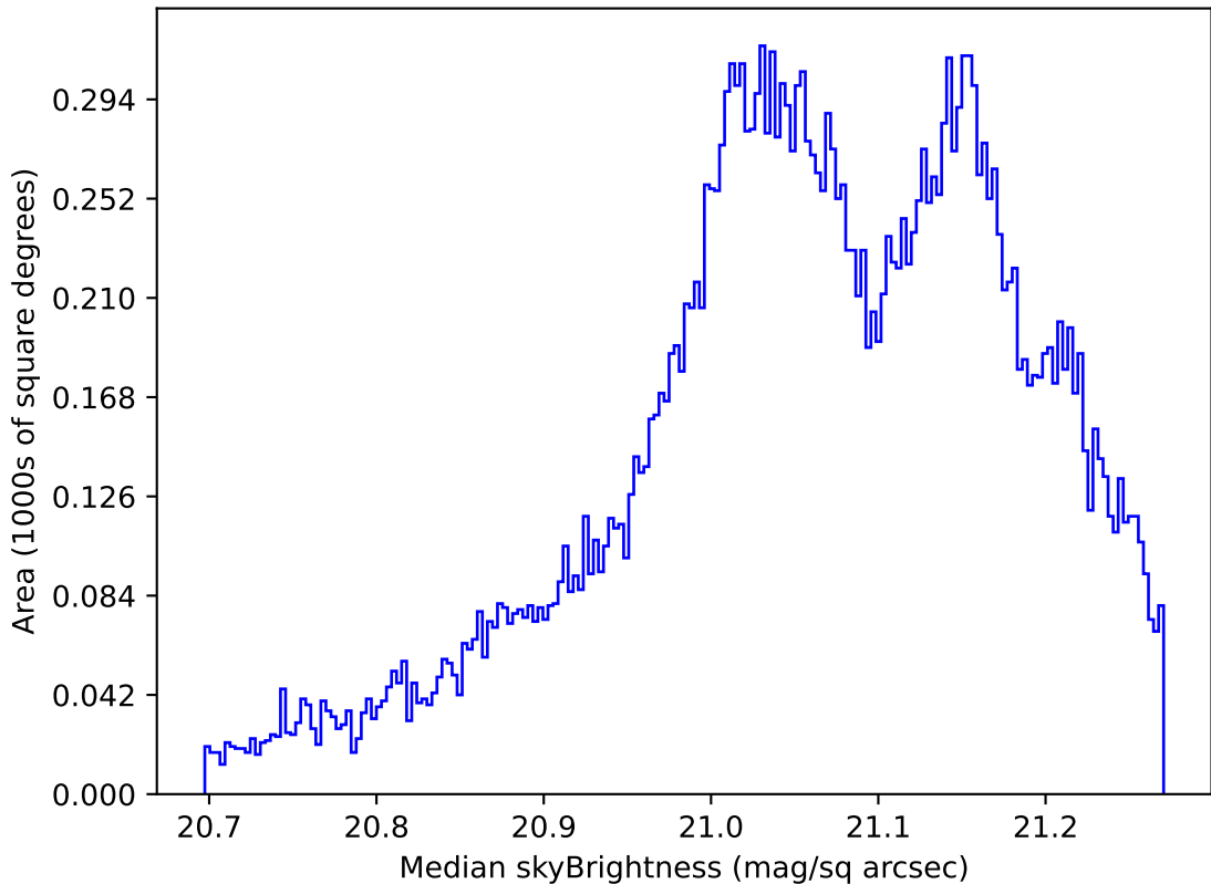
ddf_loaded_half_fl4_v3.4_10yrs All sky r band: Median skyBrightness
