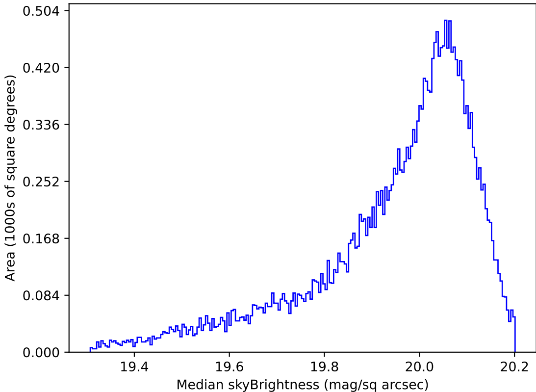
ddf_loaded_half_fl4_v3.4_10yrs All sky i band: Median skyBrightness
