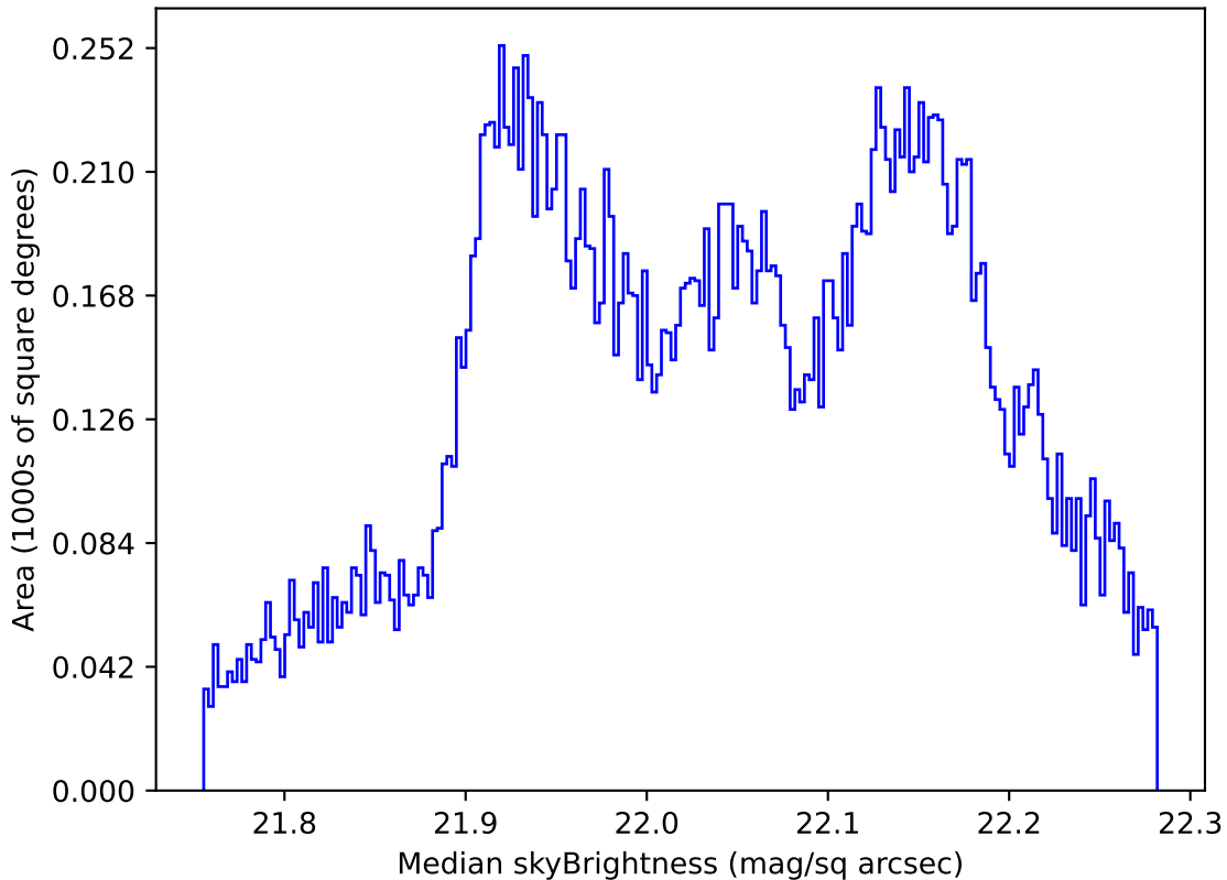
ddf_loaded_half_fl4_v3.4_10yrs All sky g band: Median skyBrightness
