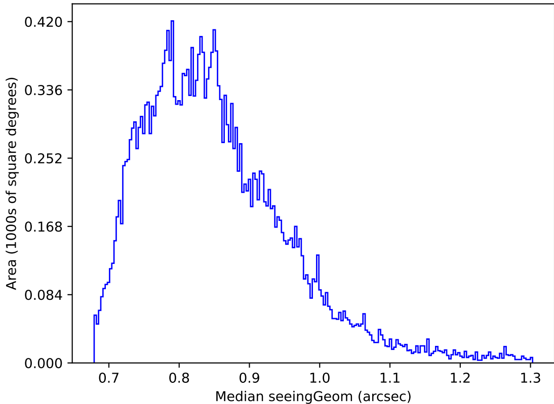
ddf_loaded_half_fl4_v3.4_10yrs Yr 1 z band: Median seeingGeom
