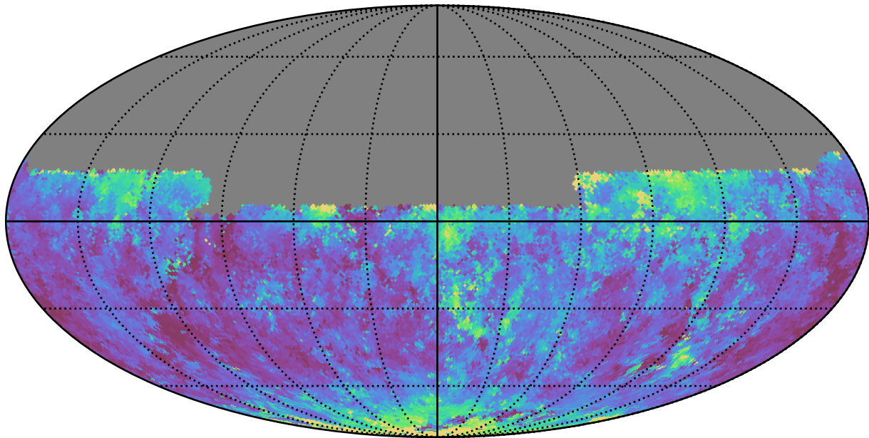
ddf_loaded_half_fl4_v3.4_10yrs Yr 1 y band: Median seeingGeom
