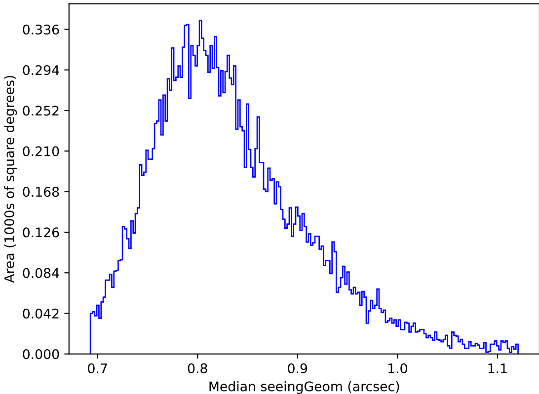
ddf_loaded_half_fl4_v3.4_10yrs Yr 1 y band: Median seeingGeom
