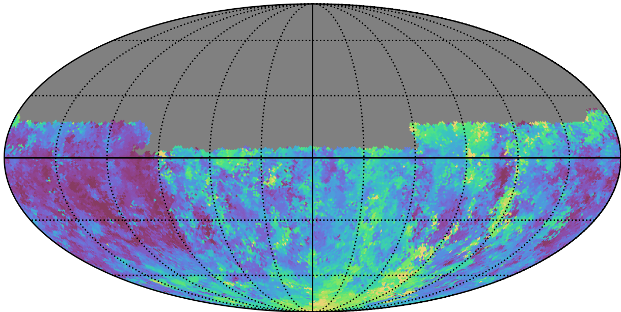
ddf_loaded_half_fl4_v3.4_10yrs Yr 1 u band: Median seeingGeom
