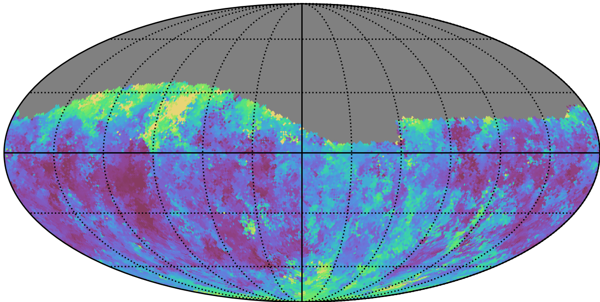
ddf_loaded_half_fl4_v3.4_10yrs Yr 1 g band: Median seeingGeom
