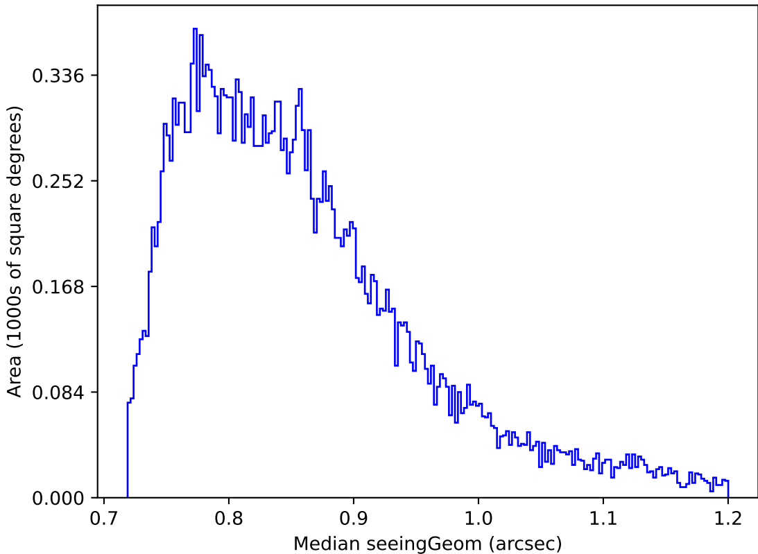
ddf_loaded_half_fl4_v3.4_10yrs Yr 1 all bands: Median seeingGeom
