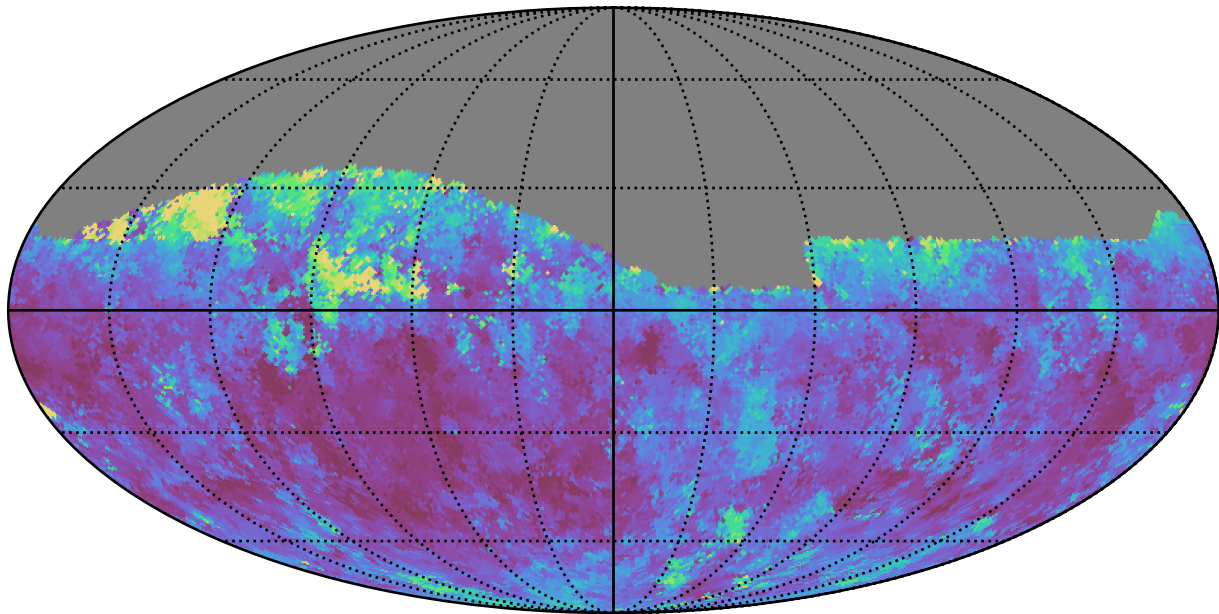
ddf_loaded_half_fl4_v3.4_10yrs Yr 1 z band: Median seeingEff
