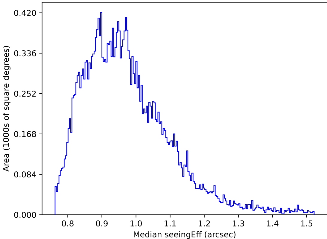
ddf_loaded_half_fl4_v3.4_10yrs Yr 1 z band: Median seeingEff
