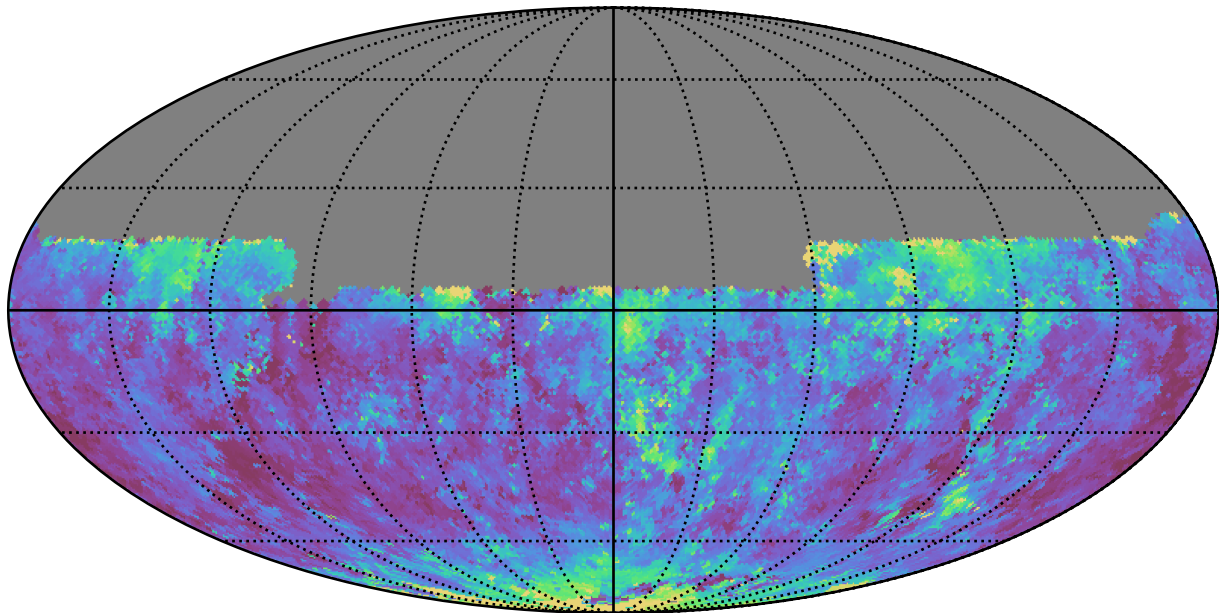
ddf_loaded_half_fl4_v3.4_10yrs Yr 1 y band: Median seeingEff
