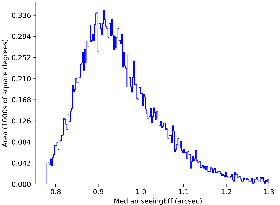
ddf_loaded_half_fl4_v3.4_10yrs Yr 1 y band: Median seeingEff
