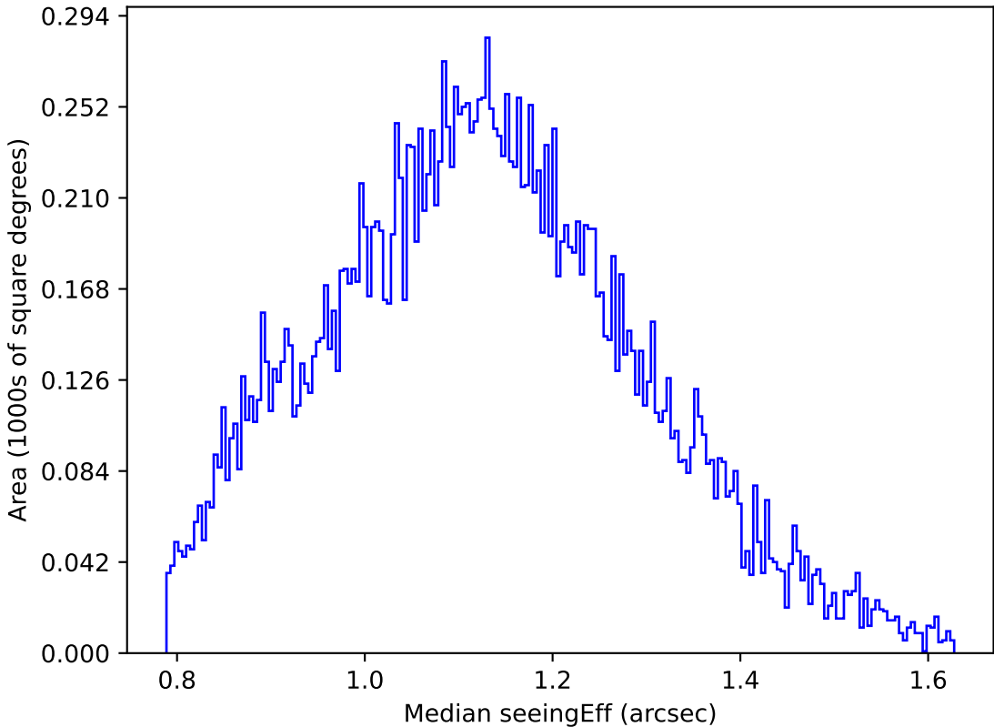
ddf_loaded_half_fl4_v3.4_10yrs Yr 1 u band: Median seeingEff
