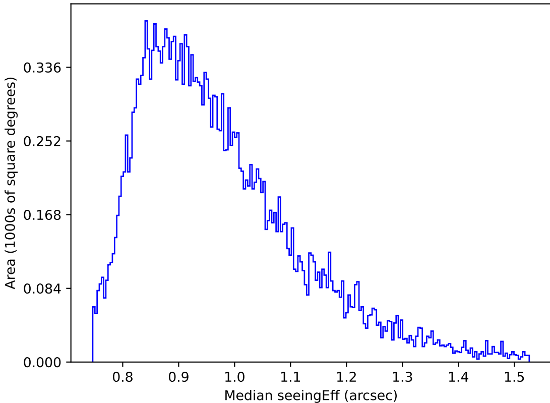
ddf_loaded_half_fl4_v3.4_10yrs Yr 1 r band: Median seeingEff
