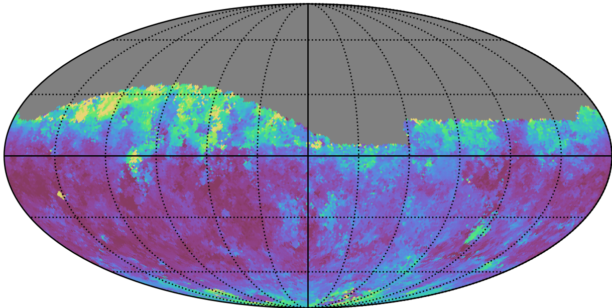
ddf_loaded_half_f14_v3.4_10yrs Yr 1 i band: Median seeingEff
