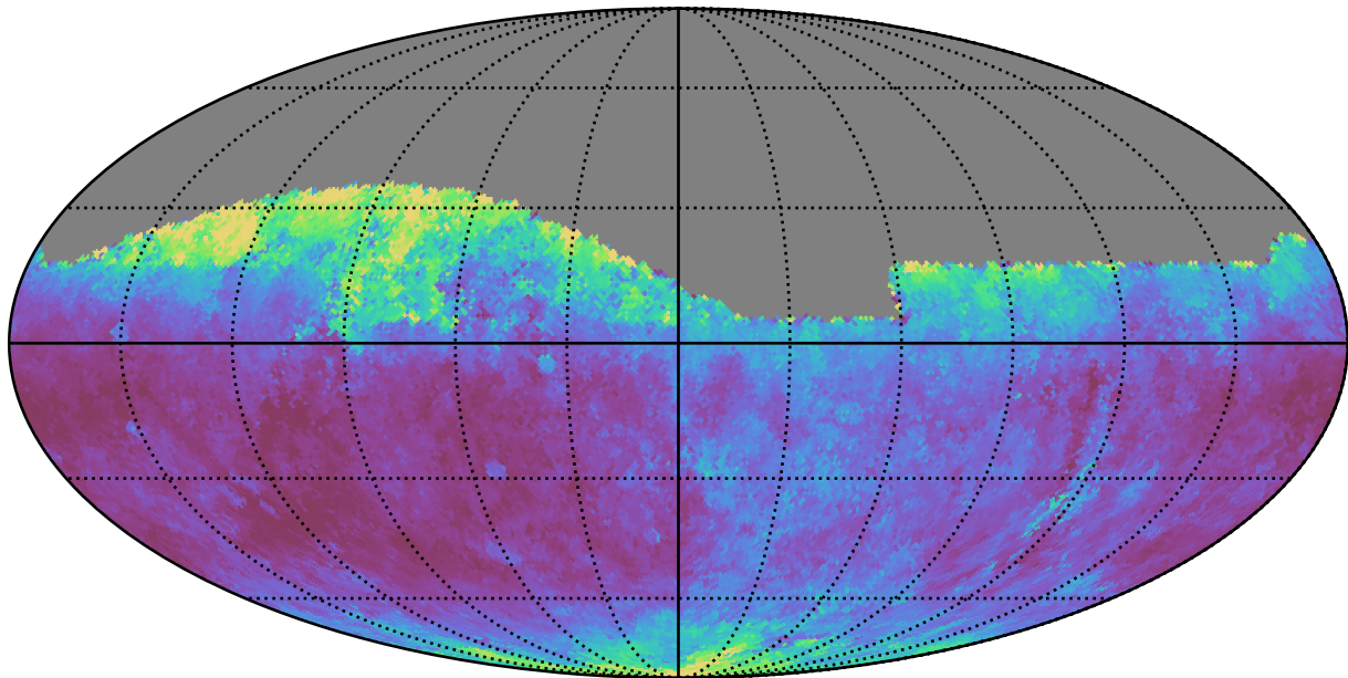
ddf_loaded_half_fl4_v3.4_10yrs Yr 1 all bands: Median seeingEff
